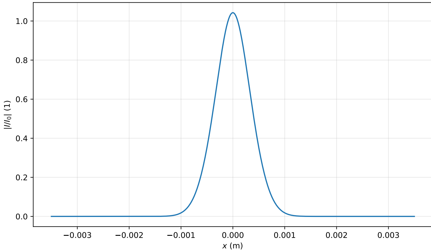
Intensity profile I(x, y = 0, z = 0.318m)/I_0 , P_{in}=0.7P_{cr} , artificial time
